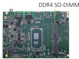
M.2 Key B ▲ Rear view
